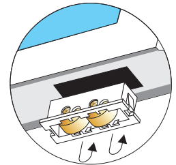
WHEEL CARRIAGE w/ adjustable brass rollers
